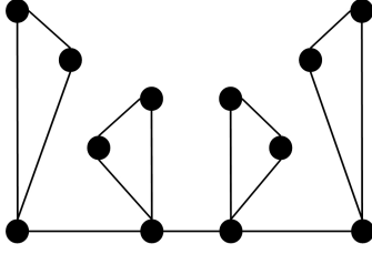
Figure 1: The rooted product graph P_4 \circ C_3 .
